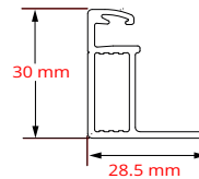
LONG SIDE FRAME PROFILE
