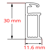
SHORT SIDE FRAME PROFILE
