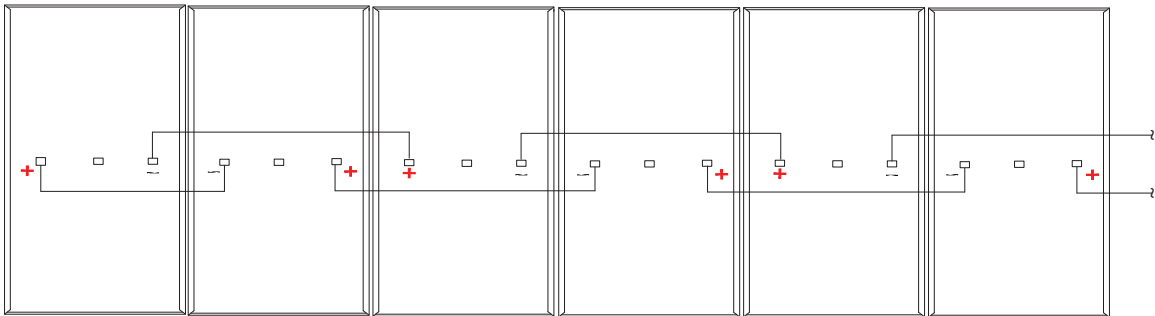
Landscape Stringing
