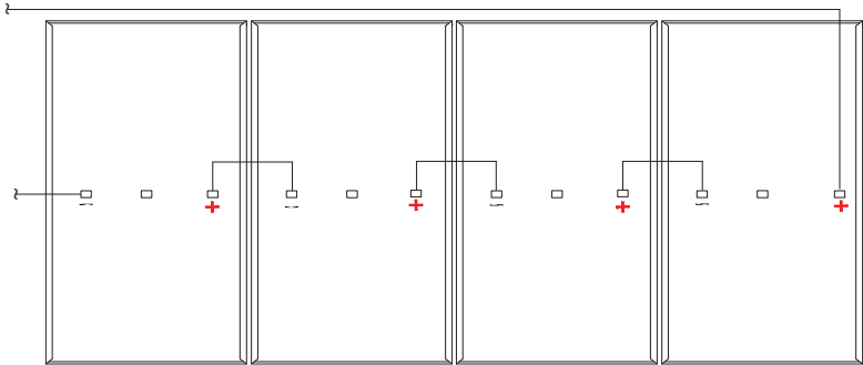
Leapfrog Stringing (Portrait)
